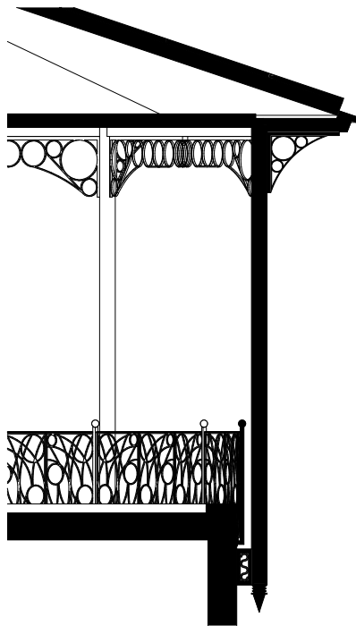
Details - 1:75
